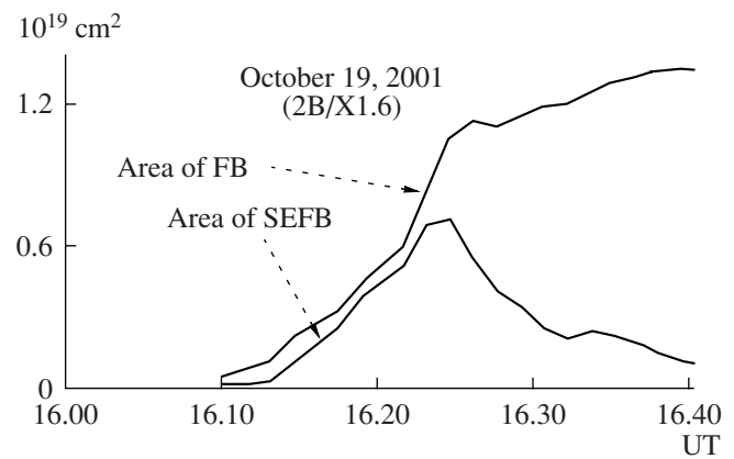
Fig. 5. The time behavior of the area of chromosphere structures, FB and SEFB.
