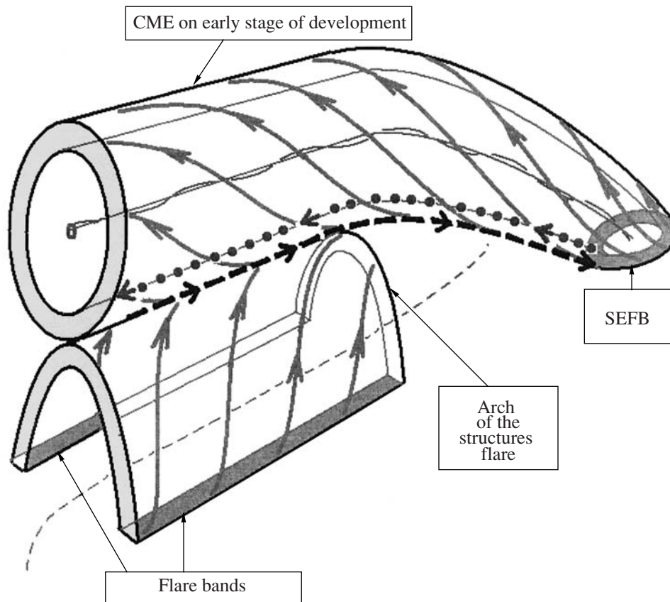
Fig. 3. The topological scheme of the solar event “flare–CME” at the early stage of its development.
