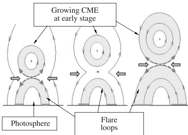
Fig. 4. Cross section of the arcade of flare loops and CME on the early stage. Successive involvement of the outer flare loops and outer shells of CME into the process is shown.
