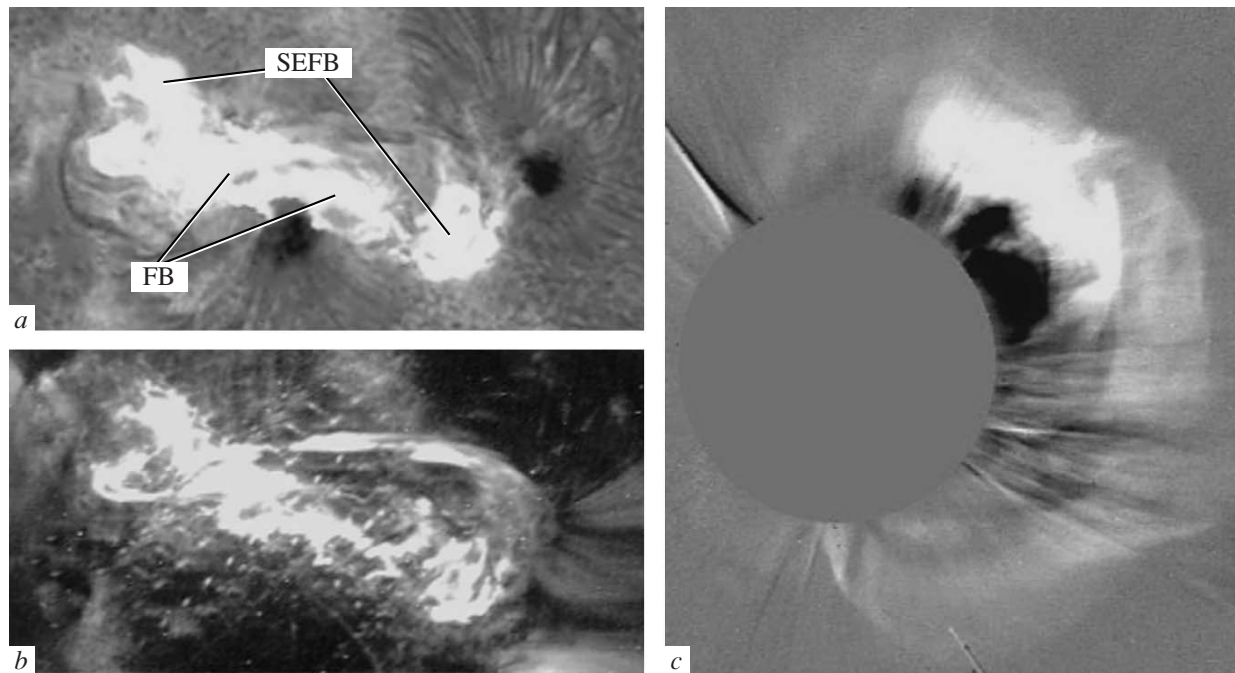
Fig. 1. The flare on October 19, 2001 on before-the maximum stage of its development (16:24 UT): (a) the image in the line H_{\alpha} (Big Bear observatory), (b) the image in the waveband 171 Å ( TRACE spacecraft). (c) The coronal mass ejection of the “halo” type detected by the SOHO spacecraft starting from 16:50 UT.
