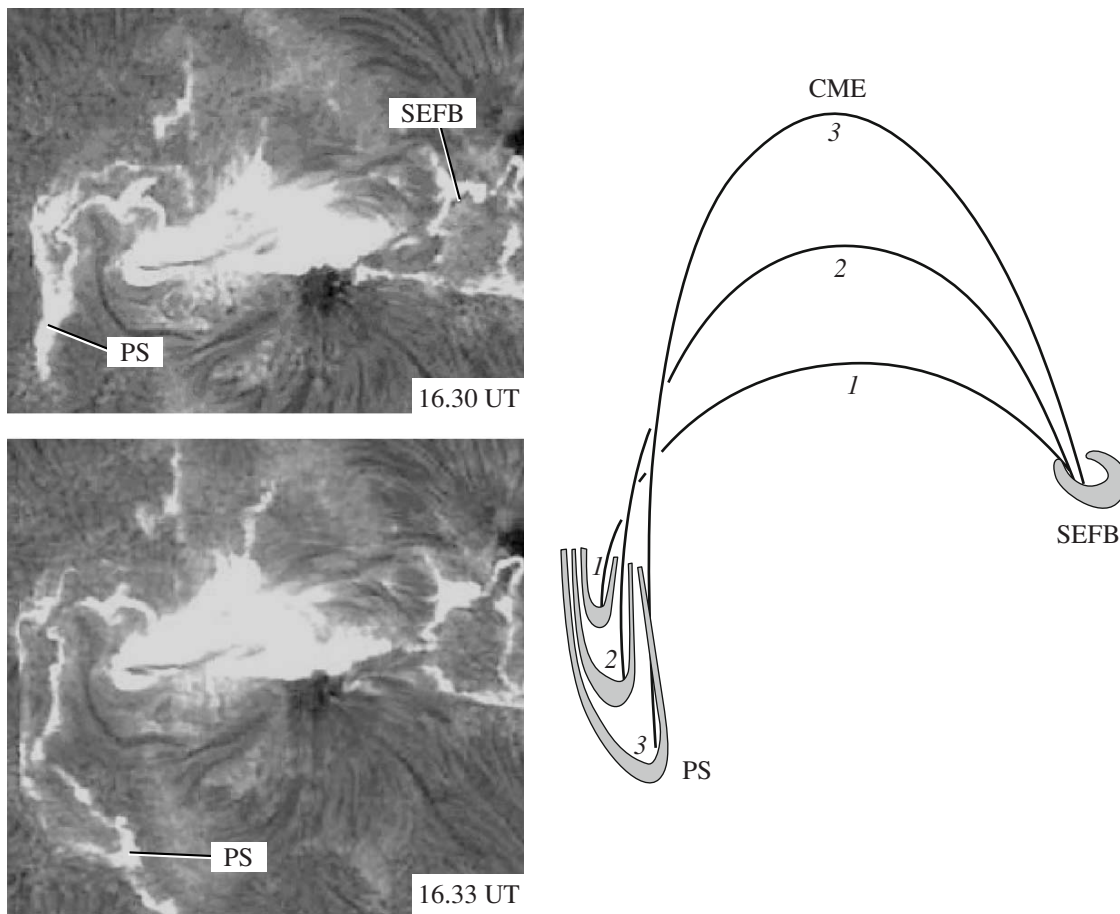
Fig. 2. Development of periphery structures during the flare (on the left) and presumable scheme of the system SEFB-PS (on the right).
