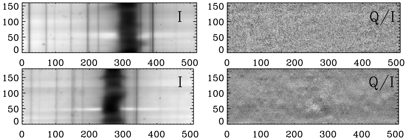
Fig. 4. The two examples of Stokes parameters I (intensity, the left panels) and Q/I (linear polarisation, the right panels) measured in moustaches with insignificant polarization ( the top panel ) and noticeable polarization ( the bottom panel ).
