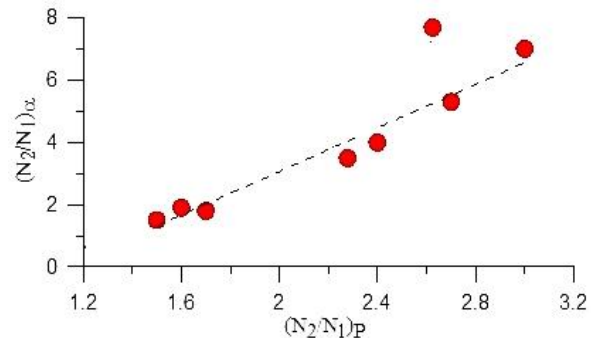
Figure 11. A relative jump in alpha-particle density (N_2/N_1)_\alpha as a function of a relative jump in proton density (N_2/N_1)_p at the front of interplanetary shock waves
