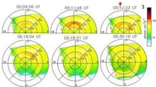
Figure 10. Magnetospheric response in auroras to the interaction with DS the source of which is the eruptive filament of the sporadic solar wind. The auroras were registered by Polar SC with an LBHL filter in the dayside polar cusp
