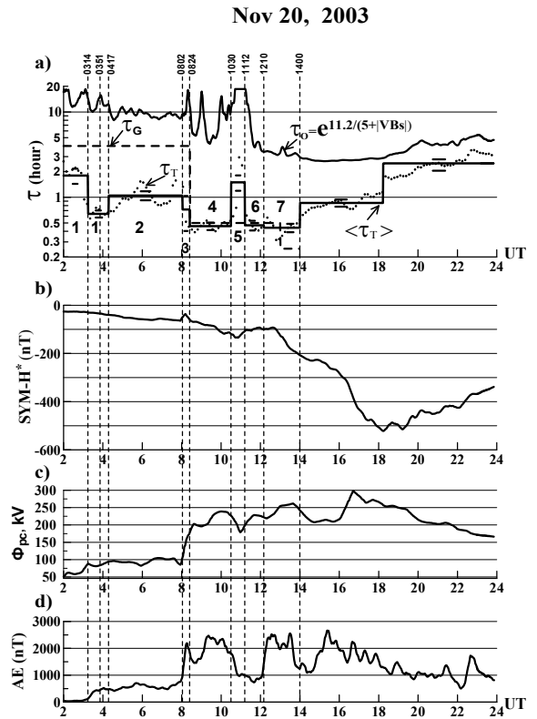
Figure 2. The D_R -current decay time: \tau_0 - after O'Brien and McPherron, \tau_G - after Gonzalez et al., \tau_T and \langle \tau_T \rangle - dotted line and solid line, that is averages for each substorm's regime marked 1 to 7 (a); SYM-H* - index corrected for solar wind dynamic pressure (b), \Phi_{PC} - the polar cap potential drop with saturation taken into account [Ebihara, et al., 2005] (c); AE - auroral activity index (d).
